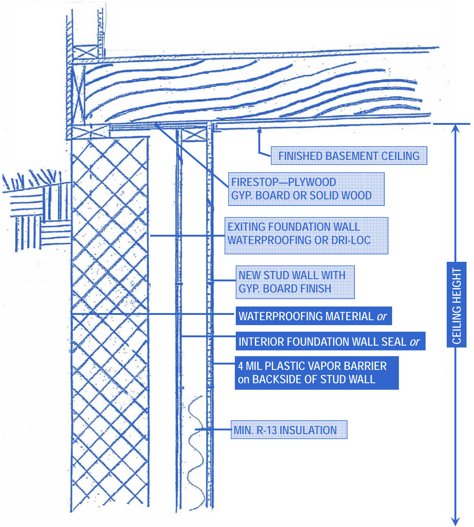
BASEMENT RENOVATION FIRESTOP DETAIL
